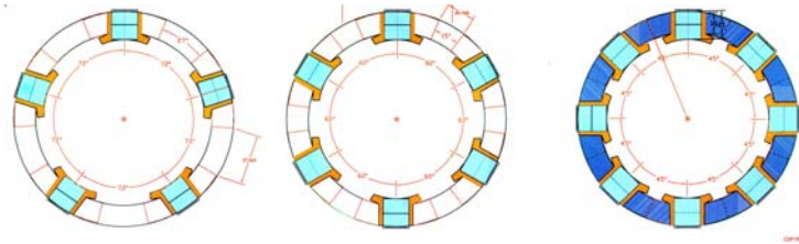
5 Channel Equidistant 6 Channel Equidistant 8 Channel Equidistant
